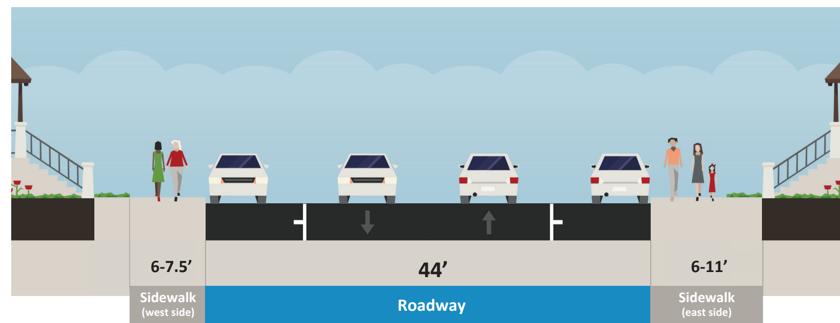
Typical Existing Cross Section
